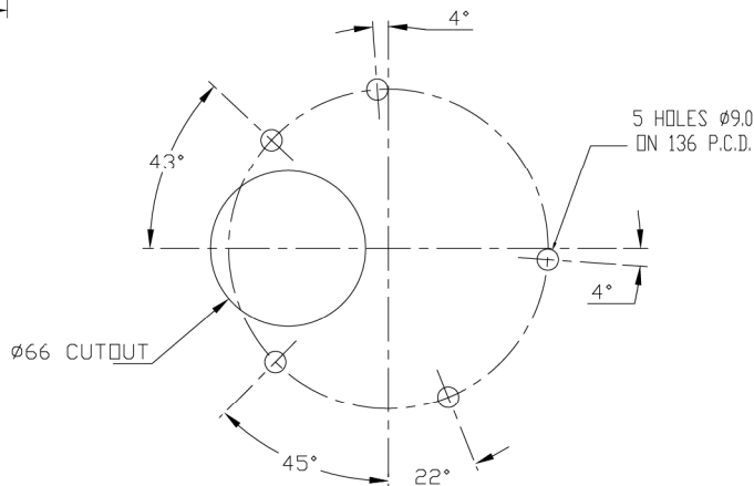
PLAN VIEW DECK CUTOUT
